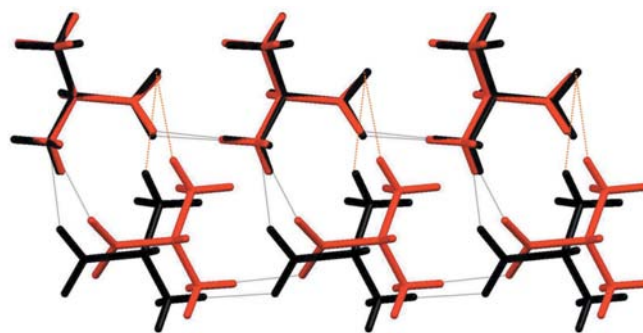
Figure 7 Superposition of the R_4^4(16) ring motifs of L-cysteine-I at ambient pressure (black) and 1.8 GPa (red). N—H···O hydrogen bonds are drawn as black dotted lines. Note the sliding movement of the layers that comprise the ring motifs over each other and a shortening of the C1—H3···O1 contact (orange dotted line) on increasing pressure as a result.
